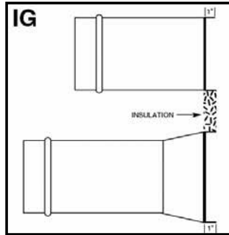
1" Insulation Guard, 26 ga., Galvanized
