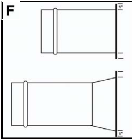
1" Flange, 26 ga., Galvanized
